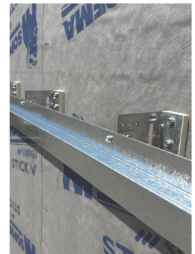
Horizontal Z-Girt
